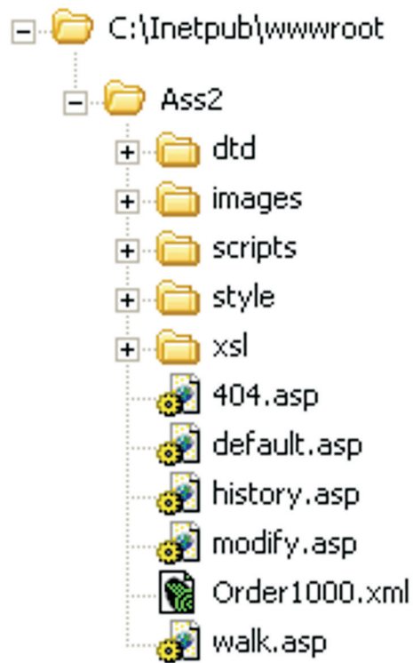
Figure 1 Directory Structure
